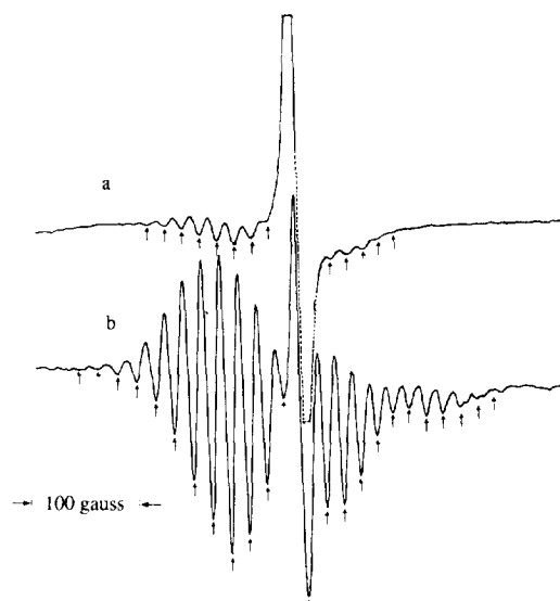
Fig. 4. ESR spectra of (a) Eu(obp)acac and (b) Eu(t-Mepyp)acac in the solid state (290 K).
