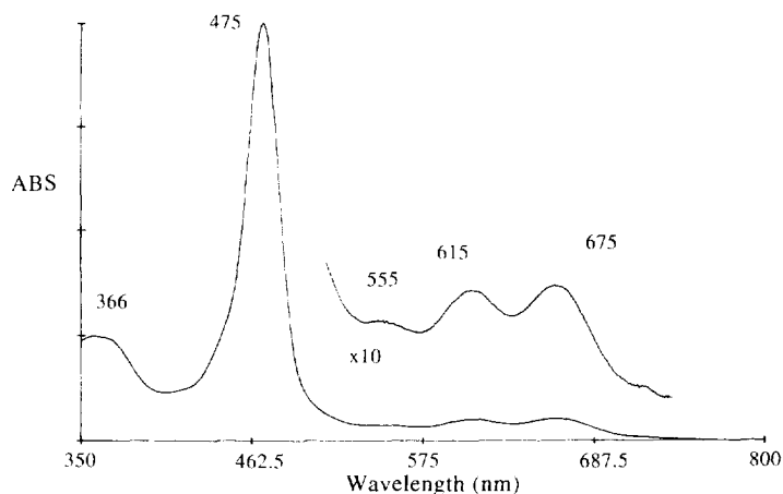
Fig. 1. UV-vis spectrum of Sm(obp)acac in CH 2 Cl 2 .
