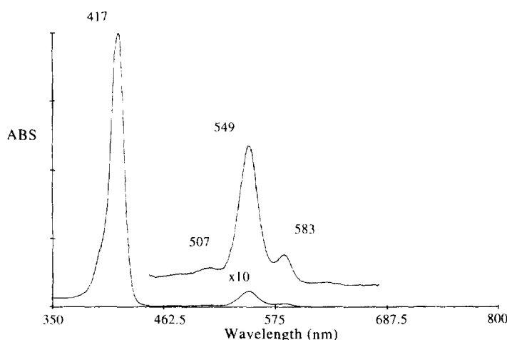
Fig. 2. UV-vis spectrum of Sm(tpfpp)acac in CH 2 Cl 2 .
